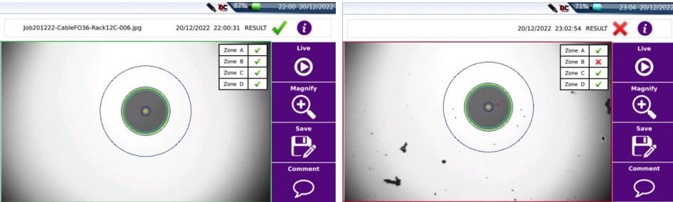
Figure 30 Scope Test results
